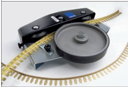
Z-FLEX CURVER
